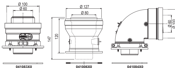
fig. 32- Starting accessories for coaxial ducts
