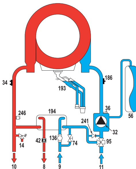
fig. 63- Hydraulic circuit
