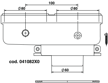
fig. 34- Starting accessory for separate ducts
