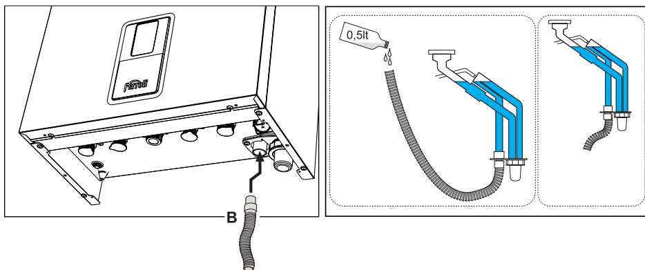
fig. 38- Condensate drain connection
