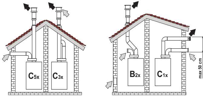
fig. 33- Examples of connection with separate pipes (⇨ = Air / ⇩ = Fumes)
