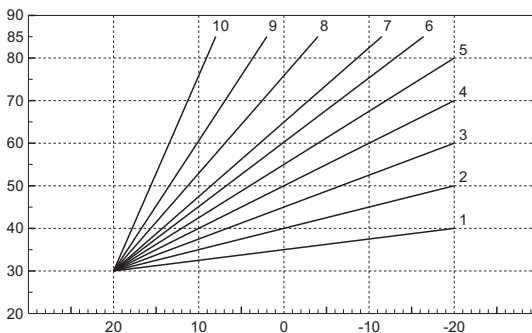
fig. 24- Compensation curves
