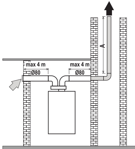
fig. 35- Layout for ducting only with flexible pipe
